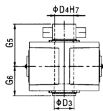
P3DV 带胀紧盘的空心轴 Hollow shaft for shrink disk
