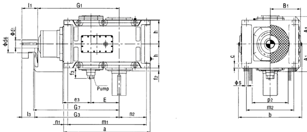
V2SV, V2HV, V2DV (强制润滑 With forced lubrication)
