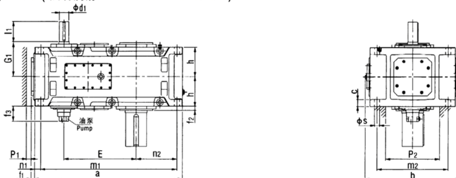
P2DV 带胀紧盘的空心轴 Hollow shaft for shrink disk
