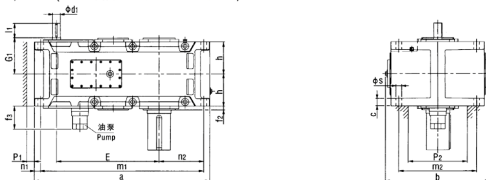
P3SV, P3HV, P3DV (强制润滑 With forced lubrication)
