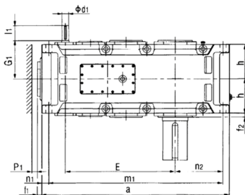
P4SV, P4HV, P4DV (强制润滑 With forced lubrication)
