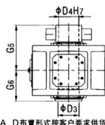
P2DV 带胀紧盘的空心轴 Hollow shaft for shrink disk
