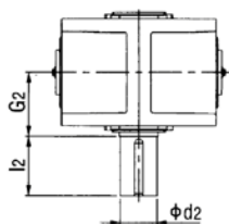
P3SV 实心轴 Solid shaft
